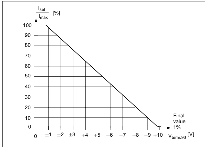
Fig. 3-4 Current setpoint limiting as a function of the voltage at 96 (R12 = open)
